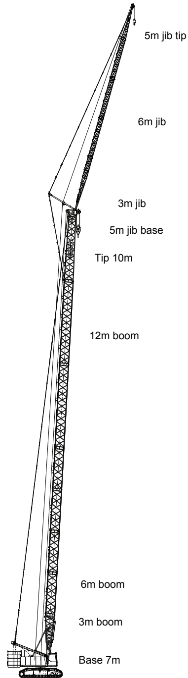
Fixed jib FJ working condition: (17m-71m) + (13m-31m)
